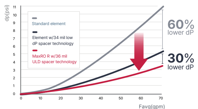
Graph A: Differential Pressure Comparison Test
